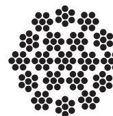
Wire Rope 7×19
