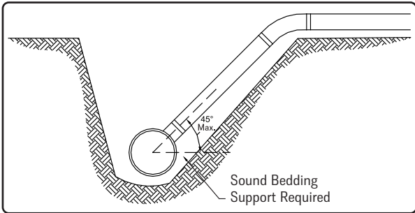
Figure 6. Service Laterals
