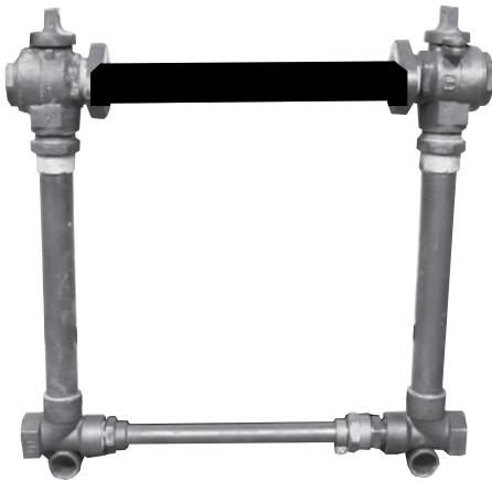
6020NL-618F6F6-UU Support bar included
