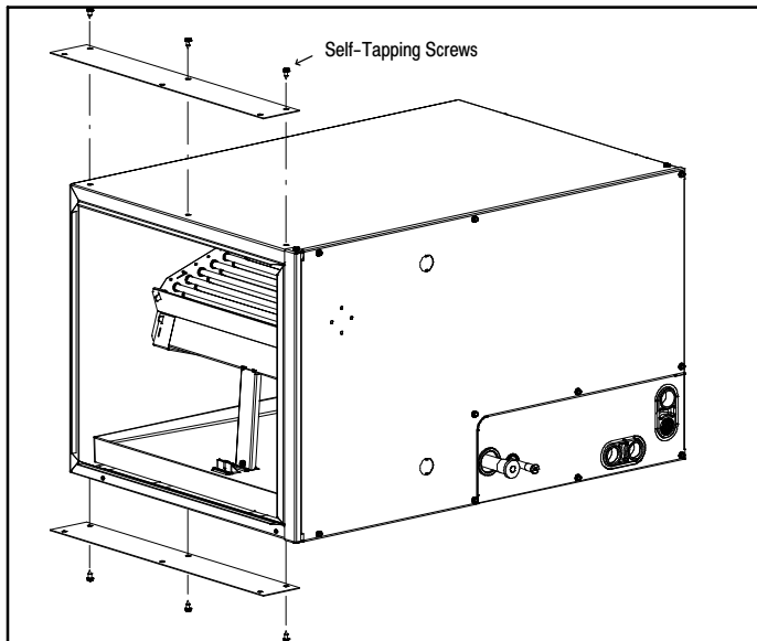
Figure 4 – Horizontal Right Installation
