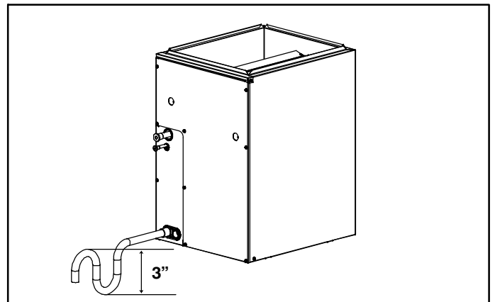
Figure 8 – Condensate Trap
