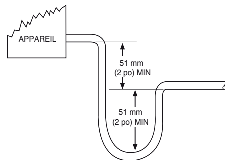
Figure 15 – Siphon de condensat recommandé
